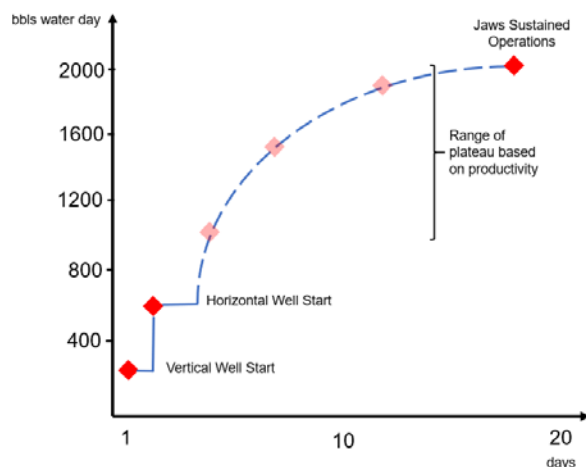
Productivity Index & Jaws Pump Plan
